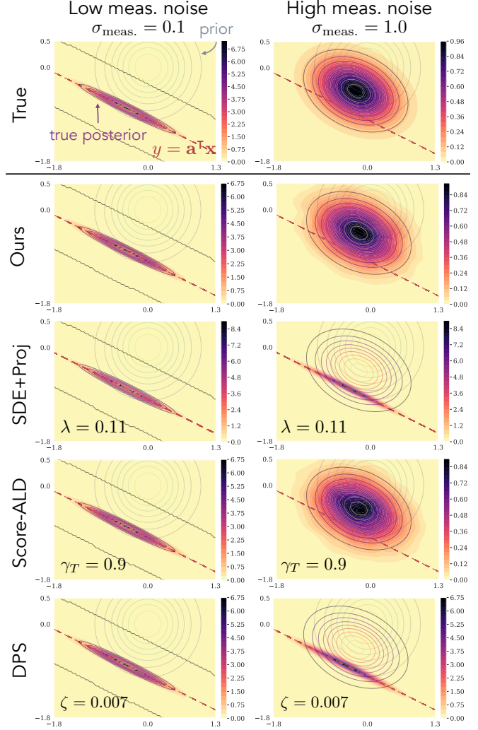
Figure 5. In this toy example with a Gaussian prior and linear measurements, we see that our method samples from the true posterior regardless of the measurement noise. For SDE+Proj, Score-ALD, and DPS, the optimal hyperparameter value was found (according to sample-approximated KL divergence to the true posterior) for the “Low meas. noise” case. The same value was then applied for the “High meas. noise” case. SDE+Proj and DPS severely underestimate the spread of the posterior. Score-ALD works well here since the approximation of the measurement-likelihood converges to the true likelihood distribution as ALD continues. In general, though, Score-ALD can become unstable when the measurement annealing rate (i.e., the sequence of \gamma_t ’s) is not well-tuned.
