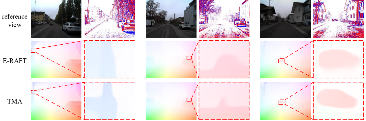
Figure 1: More qualitative results on DSEC-Flow. For each two columns, we show the reference image and event frame and compare our method with the state-of-the-art E-RAFT [2]. Significant improvements are highlighted by red boxes.
