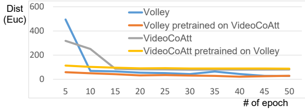
Figure 11. Learning curve of our models with pretrained models.
