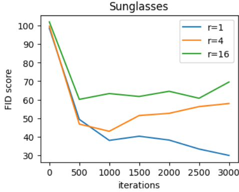
Figure 12: Comparison of FID scores in different ranks.
