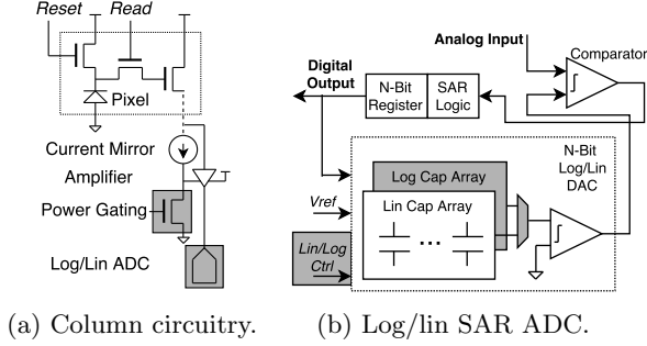
Figure 5: Our proposed camera sensor circuitry, including power gating at the column level (a) and our configurable logarithmic/linear SAR ADC (b).
