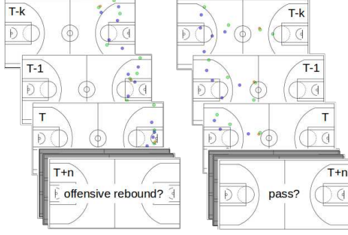
Figure 6: Examples of the basketball event prediction task: forecast an event n seconds in the future, provided a k -second history of the player and ball trajectories.
