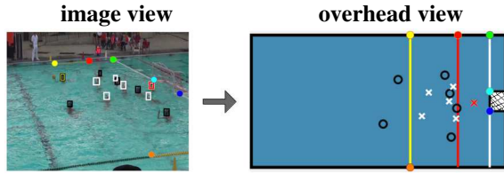
Figure 2: The image is converted into the overhead view by first estimating the homography between the image and a canonical model of the playing field using field markings such as 2m/5m lines etc. The players are then detected and their locations are transformed using the estimated homography.
