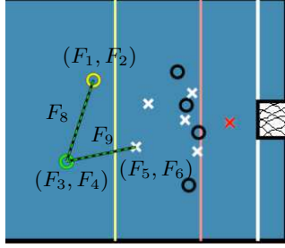
Figure 3: The features F_{[1...9]} extracted from the 2D overhead view are used to train a random forest to classify players as either receiving the ball next or not.
