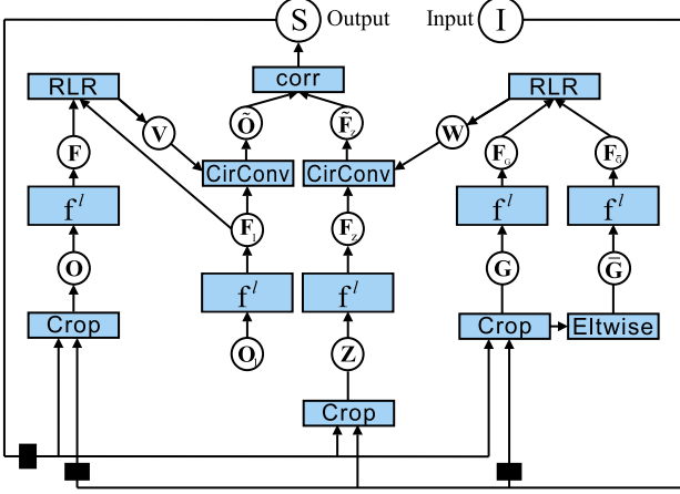
Figure 5. Network architecture of our dynamic Siamese network using single-layer deep feature f^l(\cdot) . ‘RLR’ layer represents process of learning \mathbf{V} and \mathbf{W} defined in Eq. (6) and (8). ‘CirConv’ layer denotes the circular convolution ‘ \odot ’ in Eq. (2) that leads to \hat{\mathbf{O}} = \mathbf{V} * f^l(\mathbf{O}_1) and \hat{\mathbf{F}}_Z = \mathbf{W} * f^l(\mathbf{Z}) . ‘Eltwise’ layer aims to multiply its input with a weight map and is used in section 3.3. ‘Crop’ is to get regions in image \mathbf{I} according to the position of maximum value in response map \mathbf{S} . The black block denotes a delay operation, thus we omit time index t and t - 1 in this figure.
