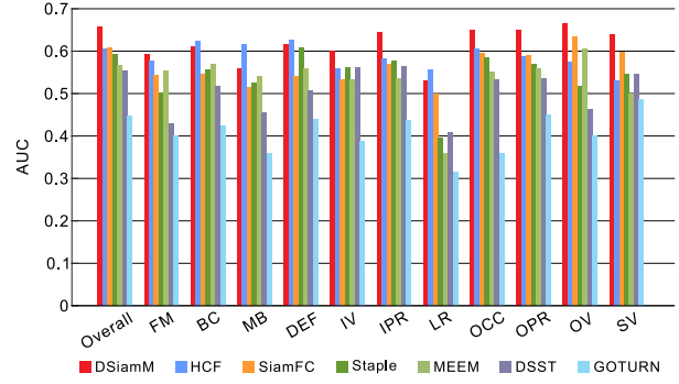
Figure 7. Specific attributes comparison of seven real-time trackers on OTB-2013 in term of success plots AUC. Our method outperforms SiamFC, Staple, MEEM, DSST and GOTURN on all 11 attributes. HCF performs better than us on attributes BC, MB, DEF and LR; while DSiamM outperforms HCF on other 7 attributes and is at least twice faster. On average, our tracker DSiamM achieves the highest accuracy among all compared real-time competitors.
