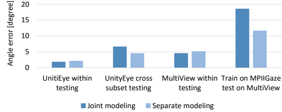
(b) Testing errors.
