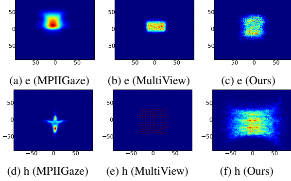
Figure 9: Eyeball movement (first line) and head pose (second line) distribution on MPIIGaze dataset [51], MultiView dataset [38] and ours.
