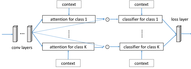
Figure 3: Detailed illustration of the context-aware attention model. For each interaction class, there is a corresponding attention model imposed on the feature map to select the interaction-specific discriminative feature regions. Different attention-pooling vectors will be generated for different interaction classes. The generated pooling vector will be then sent to the corresponding context-aware classifier to obtain the decision value.
