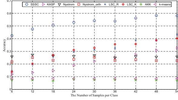
(a) Accuracy versus the different number of in-sample data
