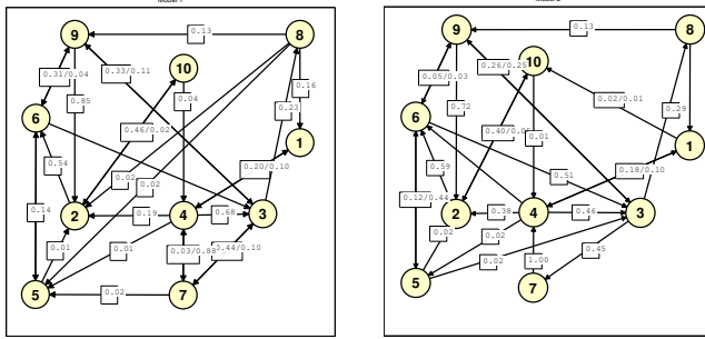
Figure 5. The two component models (Model 1 for \gamma_1 and Model 2 for \gamma_2 ) learned by the improved method, where we only draw the edges with a transition probability larger than 0.01 and ignore self transitions. The number attached to each edge indicates the transition probability.
