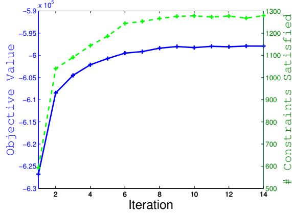
Figure 3. The convergence behavior of the improved method, where around 1250 training pairs were used. The blue curve/axis shows the value of the objective function, and the green curve/axis shows the number of constraints satisfied.
