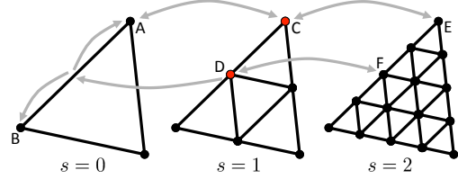
Figure 3: Adjacency across scale: C has neighbours at both finer (E) and coarser (A) subdivision. D has a neighbour at finer subdivision (F) but we consider it to have two neighbours at coarser subdivision (A and B).
