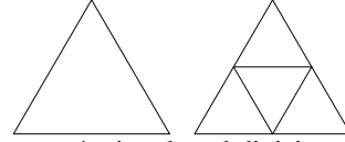
Figure 1: Aperture 4 triangle subdivision rule. By adding additional vertices to the middle of each edge, an equilateral triangle is subdivided into four equally sized triangles.
