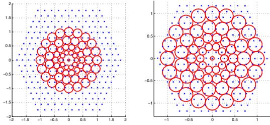
(a) Sampling octave feature. (b) Sampling intra-octave feature.
