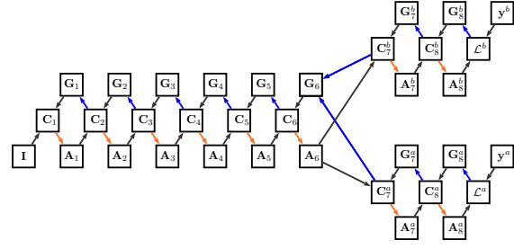
Figure 3: Memory usage in ‘vanilla’ backpropagation for multi-task training: lookup operations are indicated by black arrows, storage operations are indicated by orange and blue arrows for the forward and backward pass, respectively. During the forward pass each layer stores its activation signals in the bottom boxes. During the backward pass these activation signals are combined with the recursively computed gradient signals (top boxes).
