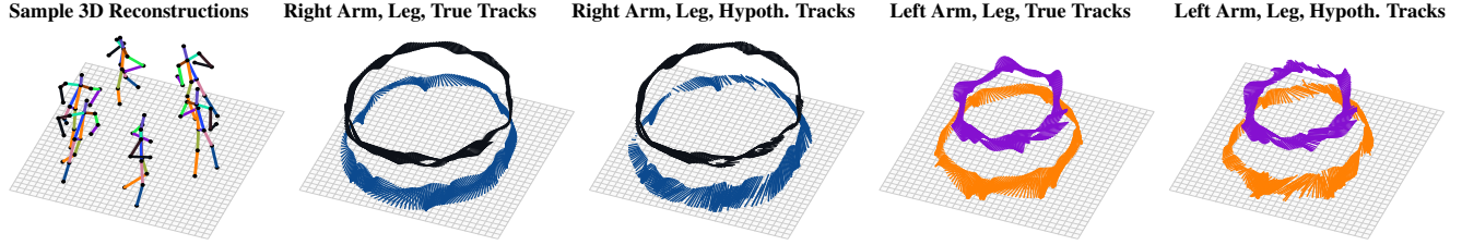
Figure 4. Hypothesizing Occluded Body Parts. Ground truth and hypothesized body parts obtained using the Fully Convolutional distance matrix regressor (Subject 3, action ‘Jogging’ from Human3.6M). The network is trained with pairs of occluded joints and is able to predict one occluded limb (2 neighboring joints) at a time. Note how the generated tracks highly resemble the ground truth ones.
