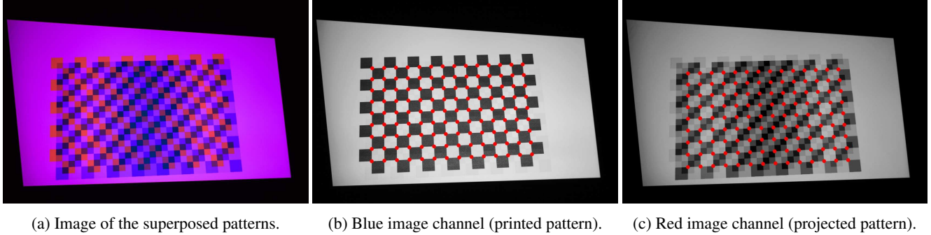
Figure 5: Captured image of an aligned superposition of the printed and the projected pattern. This is the input to step 2 of the algorithm. Corner detection for the two patterns is performed in different color channels.
