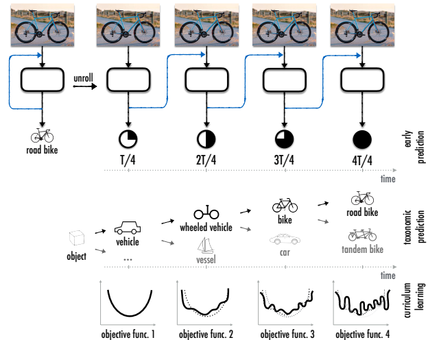
Figure 1. A feedback based learning model . The basic idea is to make predictions in an iterative manner based on a notion of the thus-far outcome. This provides several core advantages: I. enabling early predictions (given total inference time T , early predictions are made in fractions of T ); II. naturally conforming to a taxonomy in the output space; and III. better grounds for curriculum learning.
